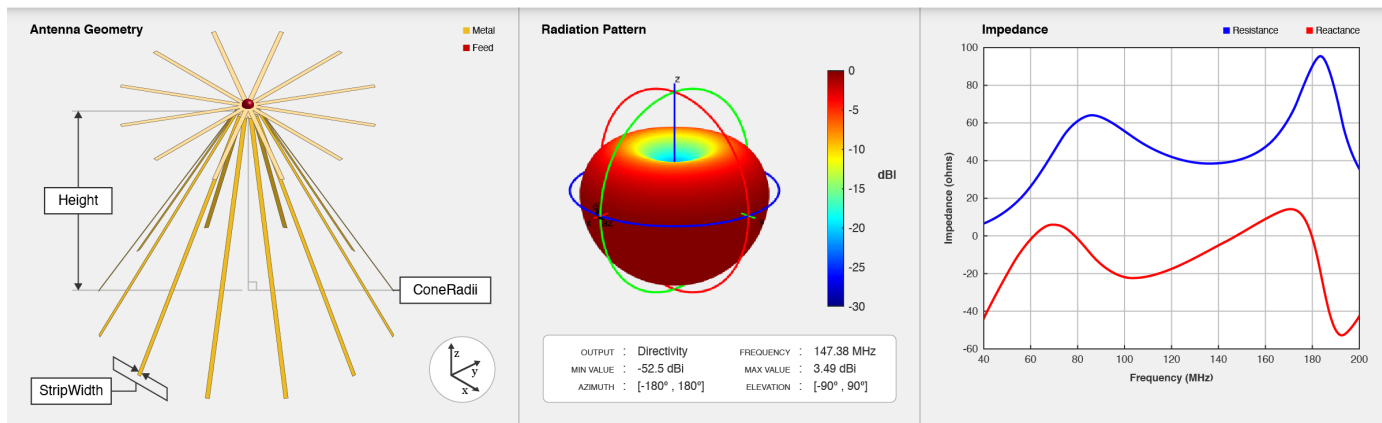
Discone Strip
